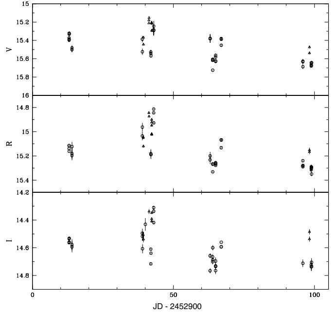
Fig. 7. Light curves of PKS 0735+17 in the V , R , I bands. The symbols are the same as in Fig. 1.
