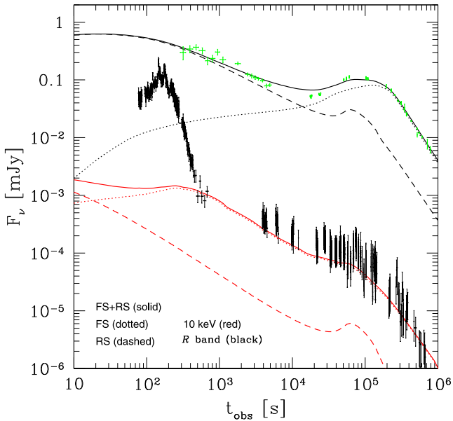
Figure 7. Results of the numerical simulation for GRB100814A X-ray and R-band light curves. RS stands for RS, while FS stands for FS emission. The prompt emission is not described by this model. For more details see Section 4.6.
