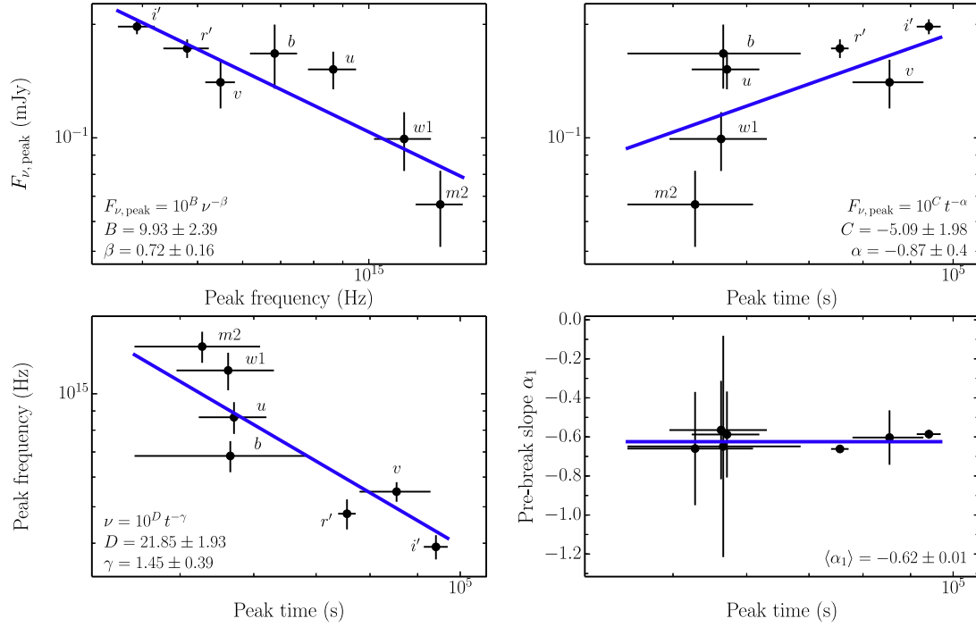
Figure 5. Relations between the peak time, t_{\text{peak}} , the peak flux density, F_{\nu, \text{peak}} , and the pre-peak slope, \alpha_1 in different UV and optical filters. The properties of the fits are summarized in Table 4.
