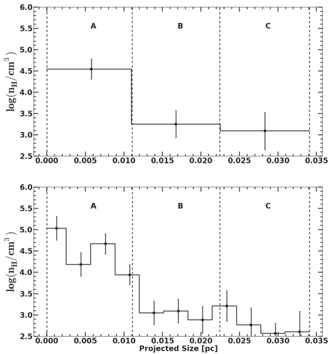
Figure 10. The top plot displays the estimated densities of regions A, B, and C (spatial resolution of \sim 5'' or 0.01 pc) from the PDR model of DB96. The solid line shows the estimate densities by DB96. The bottom plot presents the estimated densities of DB96 with a spatial resolution of \sim 1'' or 0.002 pc.
