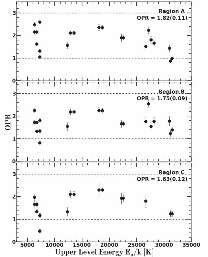
Figure 6. Plots of the OPR as a function of vibrational levels of regions A, B, and C. The dashed lines indicate the OPRs of 1 and 3. The text in the plots indicates the average OPRs of each region.
