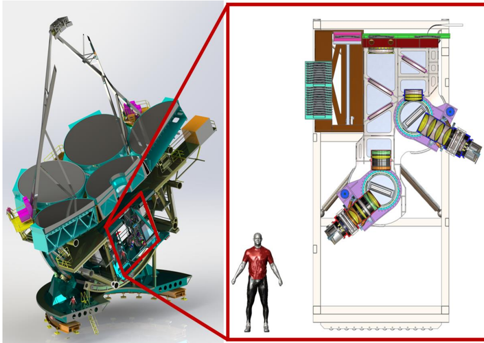
Figure 2: Rendering of the current concept for GMACS.
